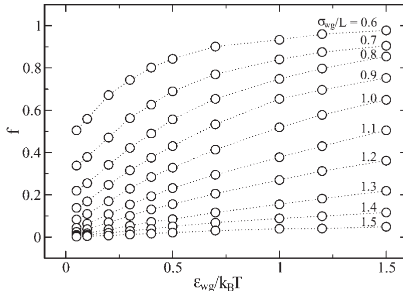
FIGURE 5 Phase diagram showing the dependence of the accommodation coefficient on the parameter \epsilon_{wg}/k_B T at various values of the parameter \sigma_{wg}/L . All the error bars are smaller than the symbols and, therefore, are not shown. The dashed lines are meant to guide the eye.
